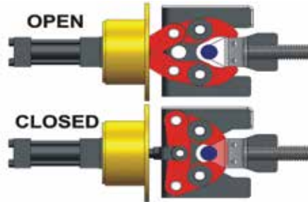
REAR HYDRAULIC CLAW DOOR Rear hydraulic claw door has an over center locking mechanism for a simple no fuss positive lock and unlock.
